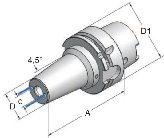
HSK - A 63
