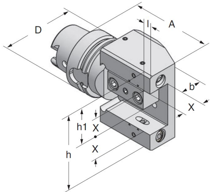
HSK - T 40
